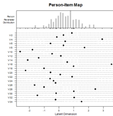
Fig 4. Person- Item Map Items of Chemistry Subject School Examination Test Instruments at SMAN 3 Tegal
