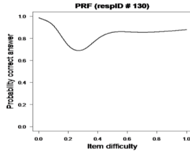
Figure 7. PRF for student no. 130 as the Copier
