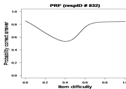
Figure 5. PRF of students detected as having DPF
