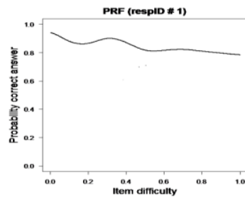
Figure 1. PRF for Consistent Response
