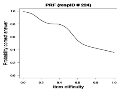
Figure 7. PRF for student no 224 as the Source
