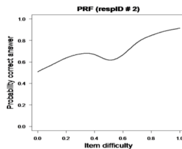
Figure 2: PRF for Abberant Response
