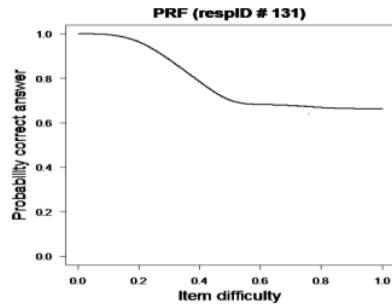
Figure 6. PRF for student no. 131 as the Source
