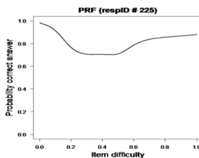
Figure 8. PRF for student no 225 as the Copier
