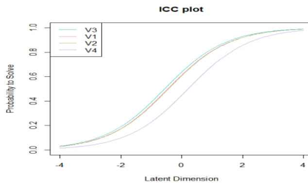
Gambar 1. Kurva Plot ICC
