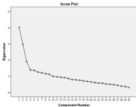
Gambar 2. Scree Plot Hasil analisis Unidimensi
