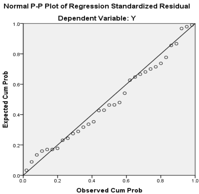
Figure 1. Normality Test
