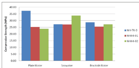
Fig. 7 Compressive strength of control specimens, M-I-K-01, and M-I-K-02 in various medias at age 28 days (modified from [9], [10])
