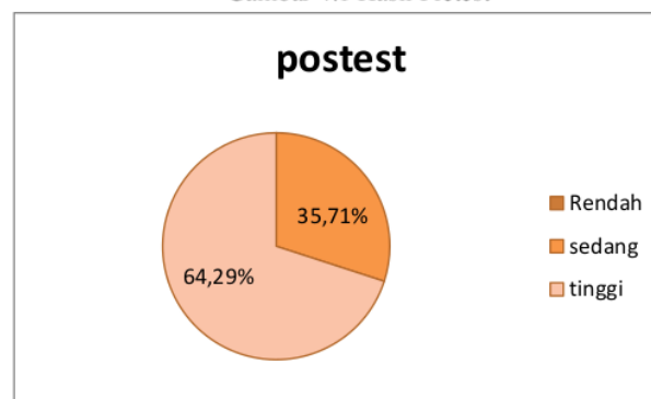
Gambar 4.2 Hasil Postest
