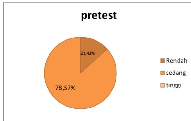
Gambar 4.1 Hasil Pretest
